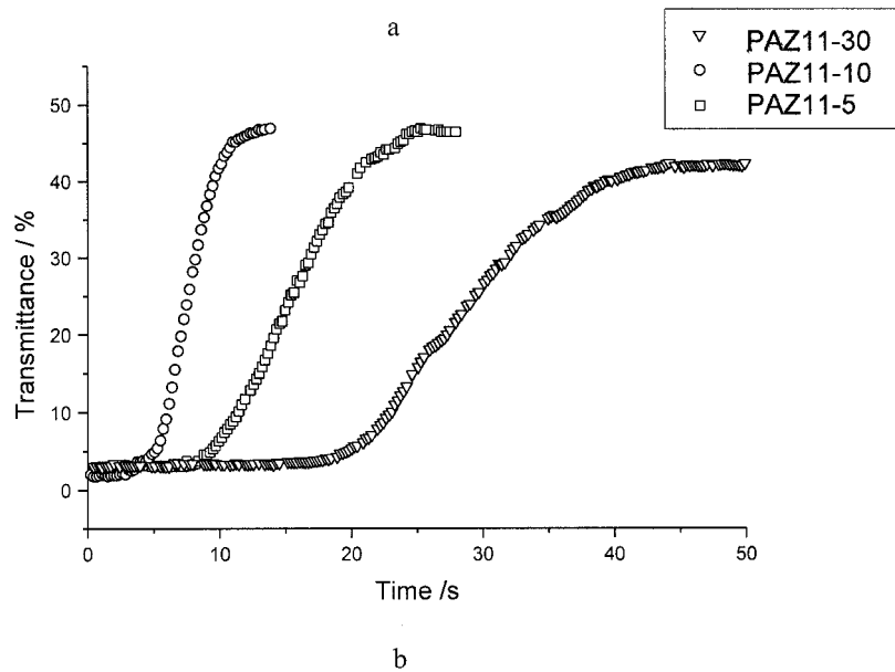
Figure 3. The effect of spacer length and azo content on the photo-driven response: PAZ3-(5, 10, 30) (a) and PAZ11-(5, 10, 30) (b) under a UV intensity of 0.5 \text{ mW cm}^{-2} at room temperature.
